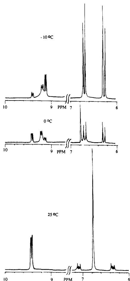
Figure 4. 1 H NMR spectra of a reaction mixture containing initially phenol (9.6 mM) and [(bpy)_2(py)Ru(O)]^{2+} (19.2 mM) in CD_3CN at -10, 0, and +25 °C. Each peak is explained in the text.
